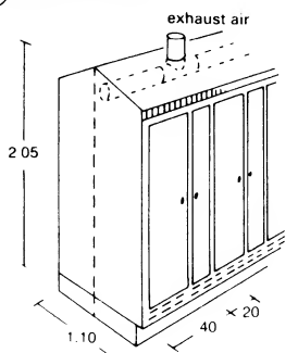
⑮ Two-compartment lockers (20 and 40 cm wide) for street and work clothes
